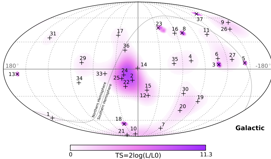
Figure 2 – High-energy starting event directions in Galactic coordinates. Cascade-like events are marked with +, track-like events with \times . The color map shows the test statistic (TS) used for the point-source clustering test at each location. Figure from 4 .
