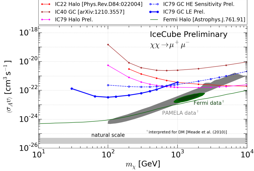
Figure 4 – 90%CL limit (w/o systematics) for WIMP annihilation in the GC into \mu^+ \mu^- (solid blue) compared to other analyses / experiments. All lines are calculated for the NFW halo model. Shown are also the regions of parameter space which provide a good fit to PAMELA (gray) and Fermi LAT (green) CR electron and positron data.
