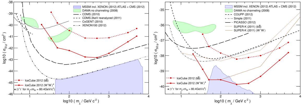
Figure 3 – 90%CL upper limits on \sigma_{SI} (left) and \sigma_{SD} (right) for the W^+W^- and b\bar{b} channels. Systematic uncertainties are included. The shaded region represents an allowed MSSM parameter space (MSSM-25) taking into account recent accelerator, cosmological and direct DM search constraints. Results from Super-K, COUPP (exponential model), PICASSO, CDMS, XENON100, CoGeNT, Simple and DAMA are shown for comparison. Figures from 8 .
