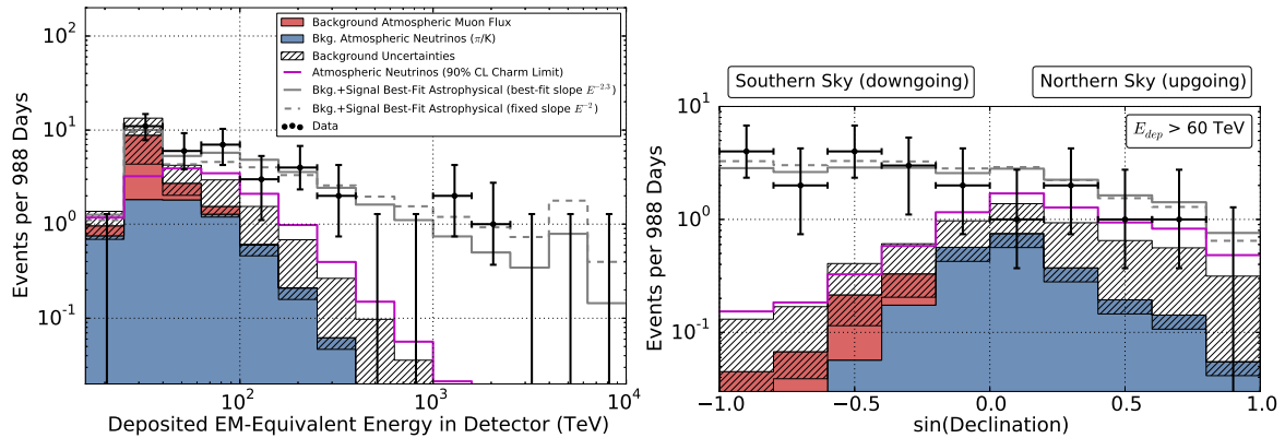
Figure 1 – Deposited energy distribution (left) and declination distribution (right) of the events observed in the 3-year high-energy starting event sample compared to background model expectations and best-fit astrophysical benchmark fluxes with fixed ( E^{-2} ) and floating ( E^{-\gamma} ) spectral indices. (Background expectations and best-fit astrophysical are stacked.) Figures from 4 .
