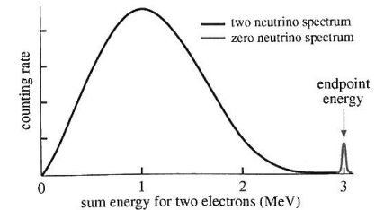
Fig. 1. Energy spectrum for the two electrons.
