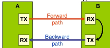
figure 2: Timing Calibration forward and backward path
