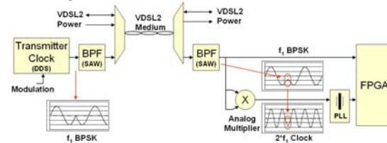
figure 3: Schematic overview of the timing calibration principle
