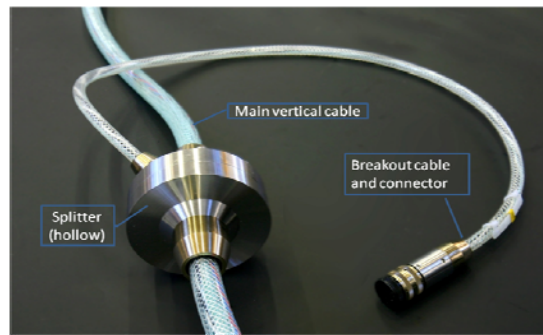
Fig. 3: Part of the vertical cable.
