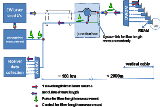
Fig. 1: Basic optical architecture
