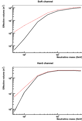
Fig. 9. Effective volume as function of neutralino mass for muons from interactions of \nu_\mu from neutralino annihilation in the Sun during the six months it is below the horizon. The dashed line corresponds to full IceCube augmented by the six Deep Core strings. The full-drawn line corresponds to full IceCube without a deep core array.
