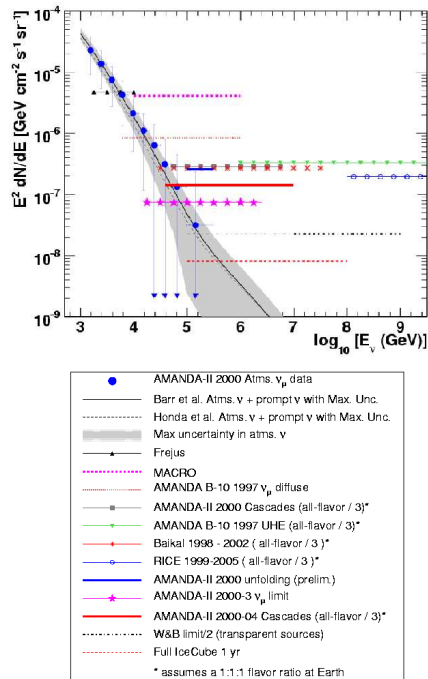
Fig. 3. Summary of existing experimental limits on the diffuse neutrino flux versus the logarithm of neutrino energy (17).
