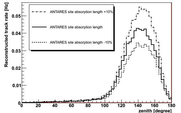
Fig. 2. Zenith distributions of reconstructed tracks using different absorption lengths. The upper (lower) histogram corresponds to an increase (decrease) of the absorption length by 10% wrt the reference values.
