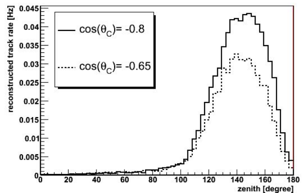
Fig. 5. Effect of the angle \vartheta_c cut-off on zenith distribution of reconstructed tracks: solid line refers to \cos(\vartheta_c)=-0.8 (reference value in MC simulation), dotted line represents \cos(\vartheta_c)=-0.65 .
