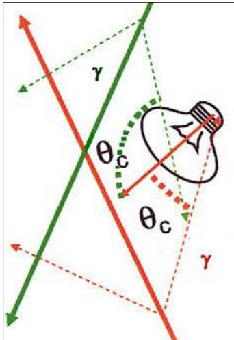
Fig. 3. Description of the angle \vartheta_c used to define the limit of detection of Cherenkov photons. Two cases corresponding to a downward going and to an upward going muon are shown.
