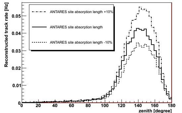
Fig. 2. Zenith distributions of reconstructed tracks using different absorption lengths. The upper (lower) histogram corresponds to an increase (decrease) of the absorption length by 10% wrt the reference values.
