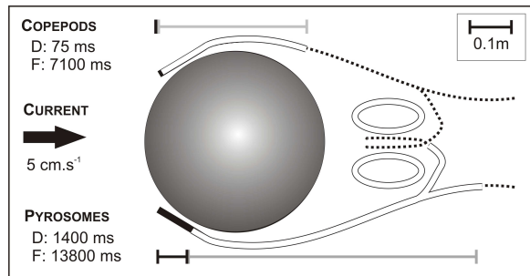
Fig.3. Hypothetical BL field produced around a sphere (43cm) by a copepod and a pyrosome advected by a current of 5\text{cm}\cdot\text{s}^{-1} . Delay (D) (■); Flash duration (F) (□); Mean flow (···)
