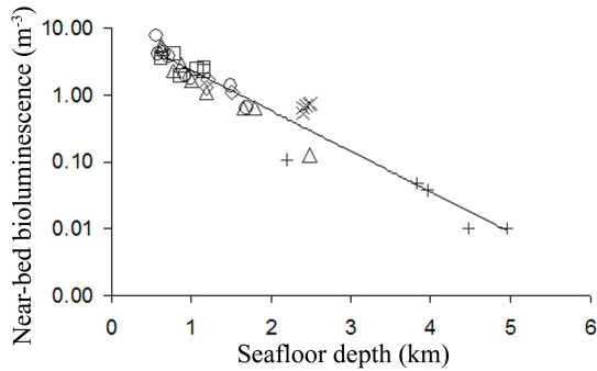
Fig.2. Plot of density of near-bed (0-400m above bottom) bioluminescence ( BL_{NB} ) ( m^{-3} ) with seafloor depth ( D_{SF} ) (km) in the: Tyrrhenian ( \diamond ); Adriatic ( \square ); NW Ionian ( \Delta ) Seas; Strait of Sicily ( \circ ); NESTOR ( + ); and ANTARES ( \times ) sites
