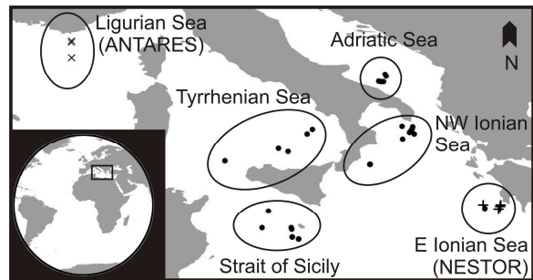
Fig. 1. ISIT-CTD profiler and ISIT free-fall lander deployment sites in the Mediterranean Sea: (x) January & May 2004; (•) October 2006 (RV Meteor M70-1); (+) May 2007 (RV Aegaeo)
