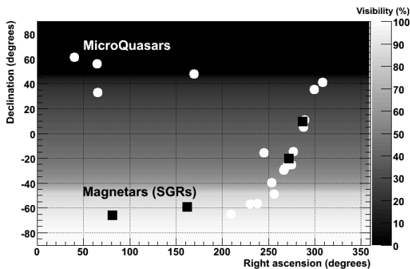
Fig. 5. Common visibility sky map for ANTARES and VIRGO.
