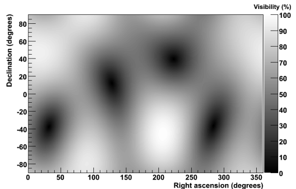
Fig. 3. VIRGO beam pattern in equatorial coordinates.
