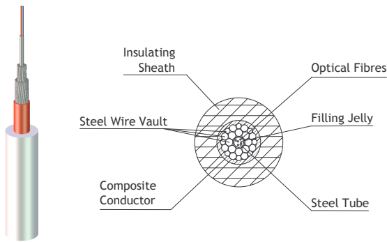
Figure 7: Deep sea cable ("Light Weight", or LW)
