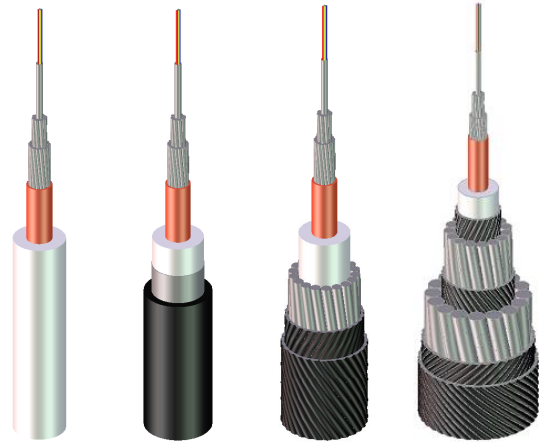
Figure 8: LW, LWP, SA, DA cable types
