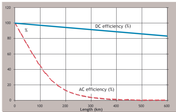
Figure 4: DC vs. AC transport efficiency
