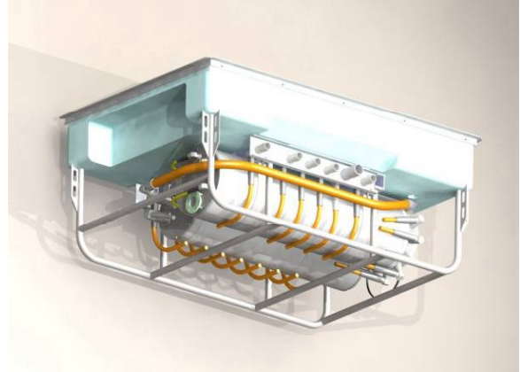
Figure 13: NEPTUNE Node Module
