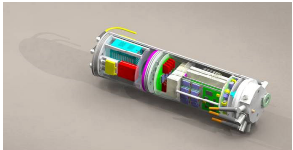
Figure 14: LV/Comms pressure vessel
