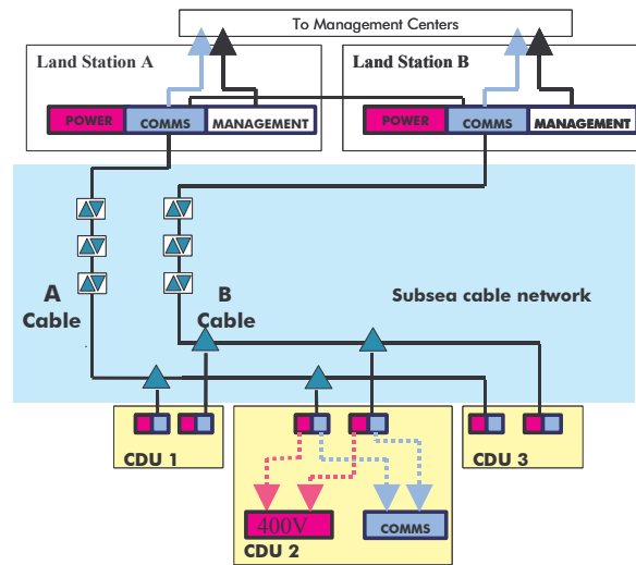
Figure 16: Preferred 1+1 architecture
