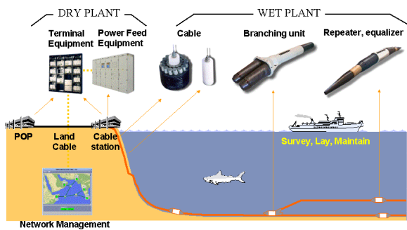
Figure 1: Repeated system schematic
