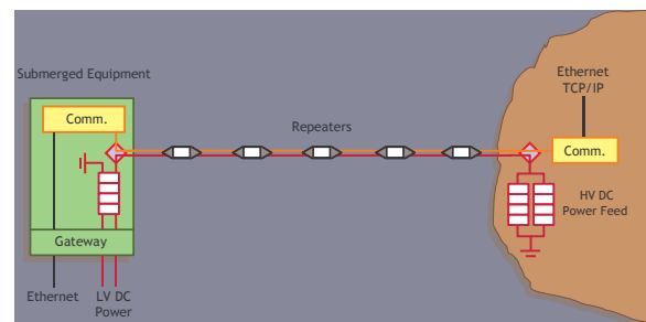
Figure 3: Subsea network principle
