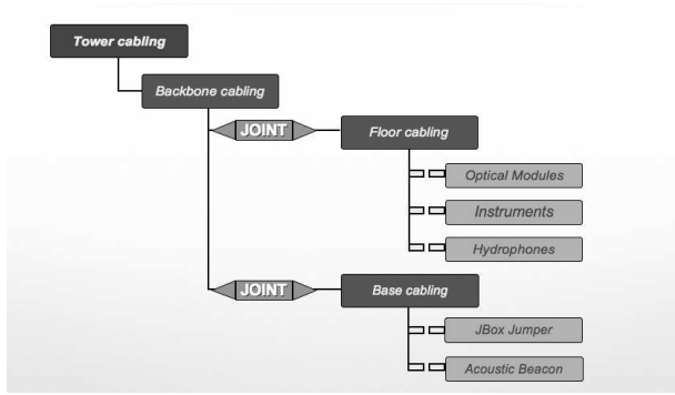
Fig. 1. Cabling system interfaces
