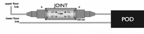
Fig. 3. Backbone joint.
