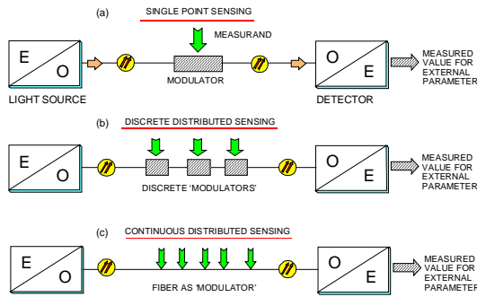
Fig. 1: Fiber-based transmission sensor configurations
