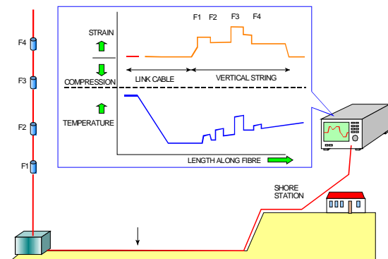
Fig. 3: Fiber-based strain and temperature sensing in a VLVnT. Inserts show examples of distributed measurements.
