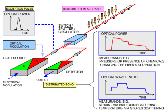
Fig. 2: Fiber-based time-domain reflectometry sensor
