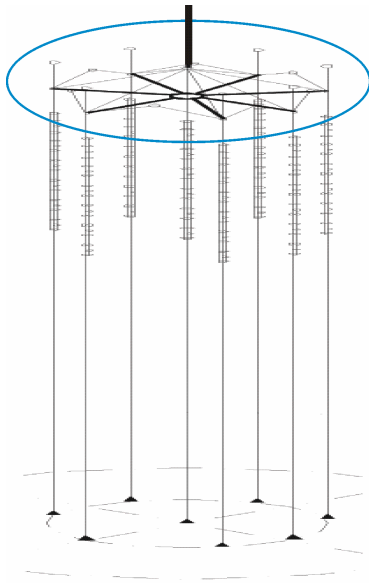
Fig. 1. Sketch of the Baikal Neutrino Telescope NT200:
