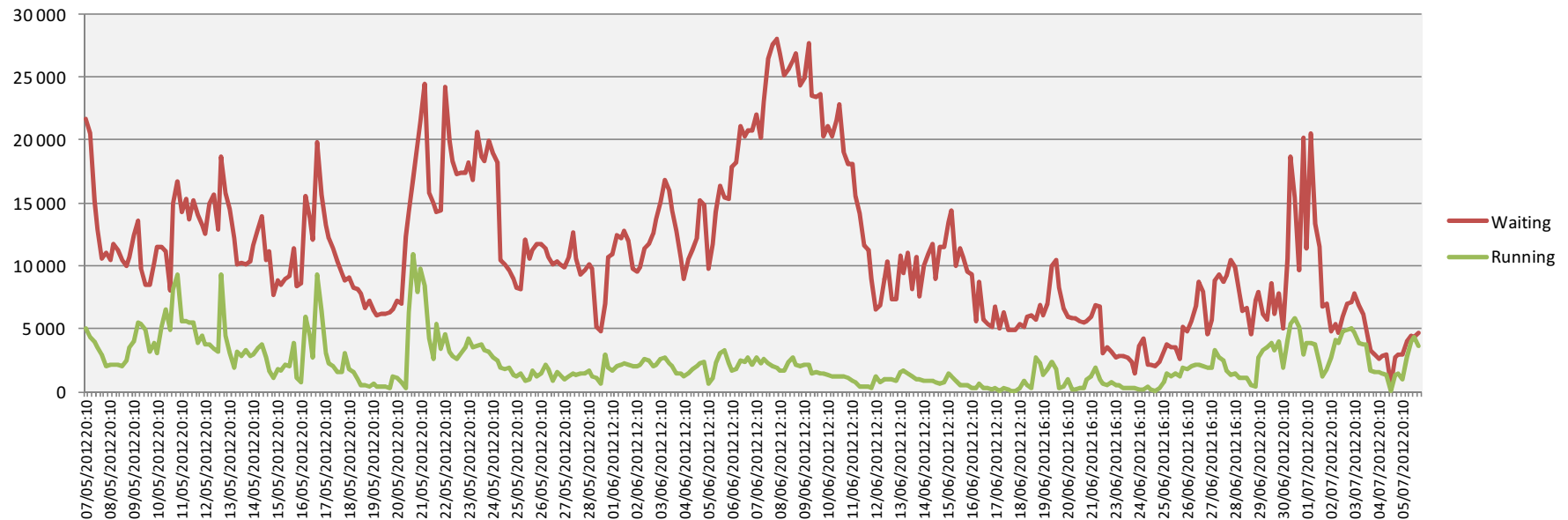
Number of jobs by status waiting/running
