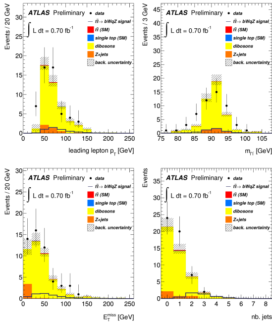
Fig. 1. Distributions obtained with the t \rightarrow qZ analysis after the preselection. Transverse momentum of the leading lepton (top left), reconstructed mass of the two leptons with same flavor and opposite charge (top right); E_T^{\text{miss}} (bottom left) and number of jets (bottom right), are shown. The background uncertainties shown include the MC simulation statistical uncertainties and the DD uncertainties. The signal distributions are normalized to the observed BR limit, at 95% CL.
