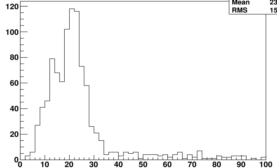
True neutrino energy
