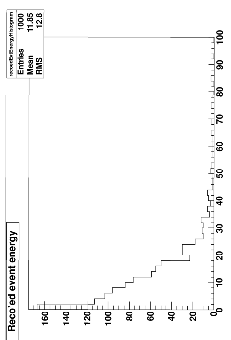
Reco'ed event energy VS true neutrino energy
