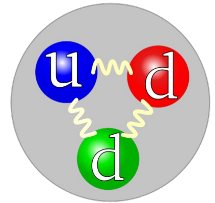
neutron
