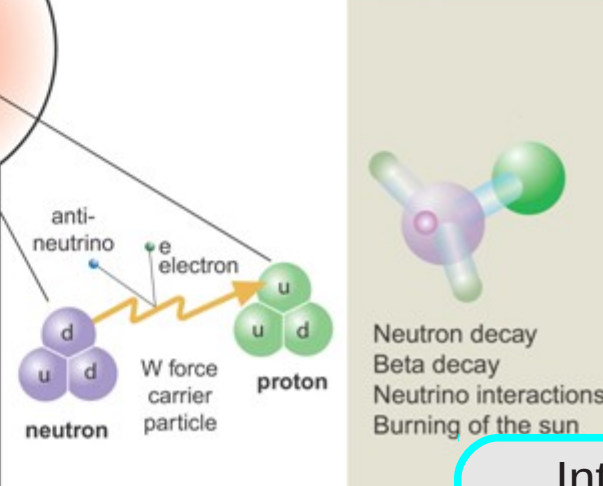
Weak force
