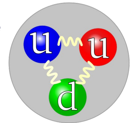
proton
