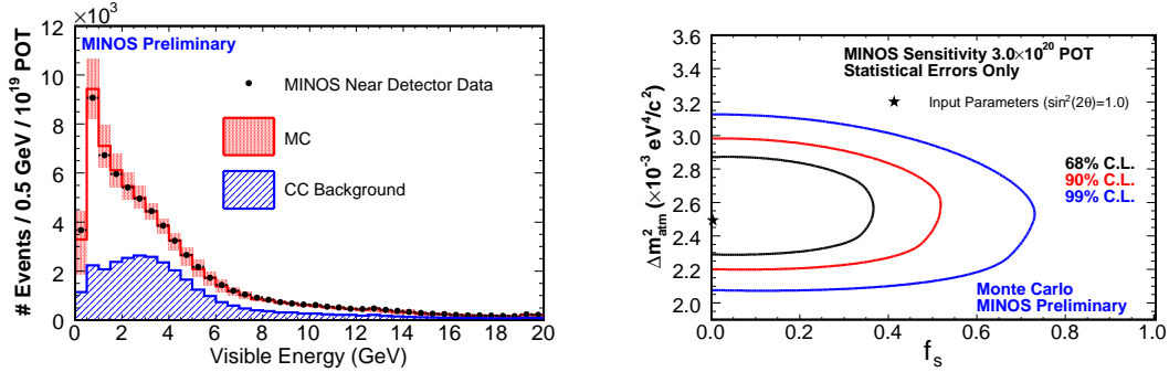
Figure 4: (Left) The spectrum of NC-selected events seen in the near detector for an exposure of 3.0 \times 10^{20} pot. The black dots are the reconstructed neutrino data, the red boxes the expected signal (systematic error bands as the area), and the blue region the expected CC contamination to this NC signal. (Right) The projected sensitivity to a fraction of \nu_m u disappearance to sterile rather than active neutrinos, as a function of \Delta m^2 .
