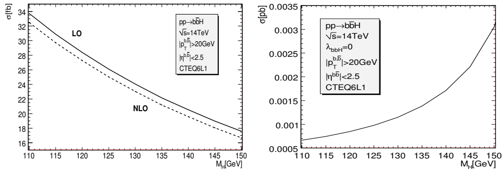
Figure 2: Left: the leading order (LO) and NLO cross sections as functions of M_H . Right: the cross section in the limit of vanishing \lambda_{bbH} .
