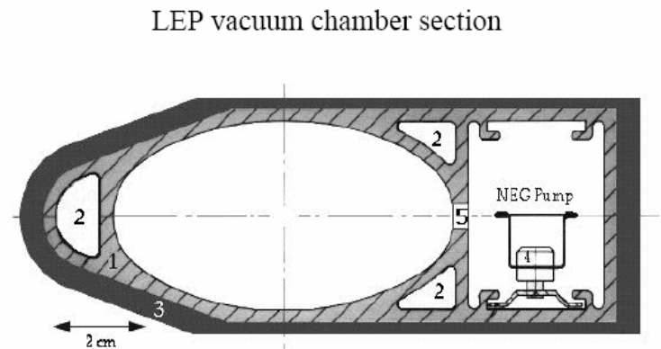
Fig. 2 : Vacuum chamber section made of (1) extruded aluminium profile with the elliptic beam channel, three cooling water ducts (2) and surrounded by 3 to 8 mm thick lead shield (3). The NEG pump (4) is housed in a separate pump channel connected to the beam channel by a row of longitudinal slots (5).
