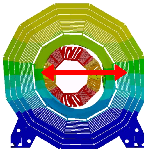
Mode 2 @ 3,05Hz
