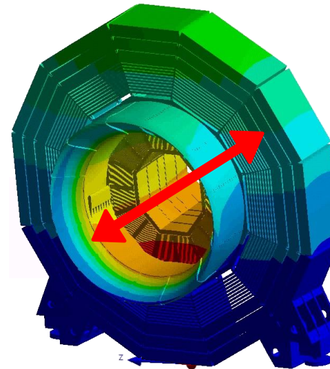
Mode 3 @ 3,8Hz
