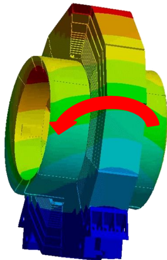
Mode 1 @ 2,3Hz
