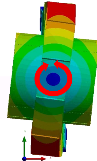
Mode 6 @ 7H
