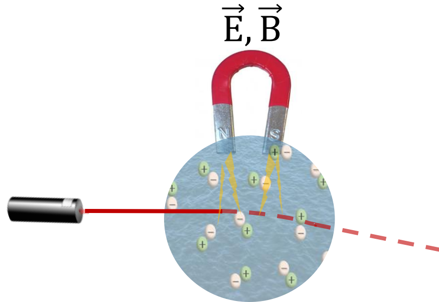
Quantum Electrodynamics Vacuum Polarisation
