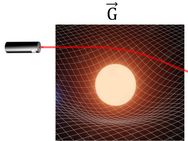
General Relativity Curvature of the metric
