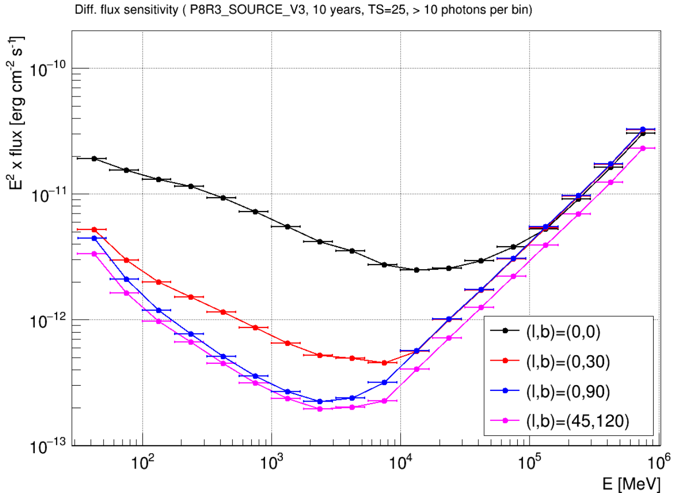
Figure 1: The Fermi-LAT point source sensitivity after 10 years of observations. The vertical axis corresponds to the value of F_0 in question 4. Adapted from https://www.slac.stanford.edu/exp/glast/groups/canda/lat_Performance.htm
