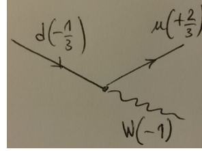
Figure 5: Example of quark-quark- W interaction.
