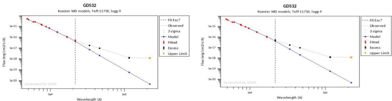
Figure 8. Plot of the SED fitting before and after refining the infrared excess (Step 8).
