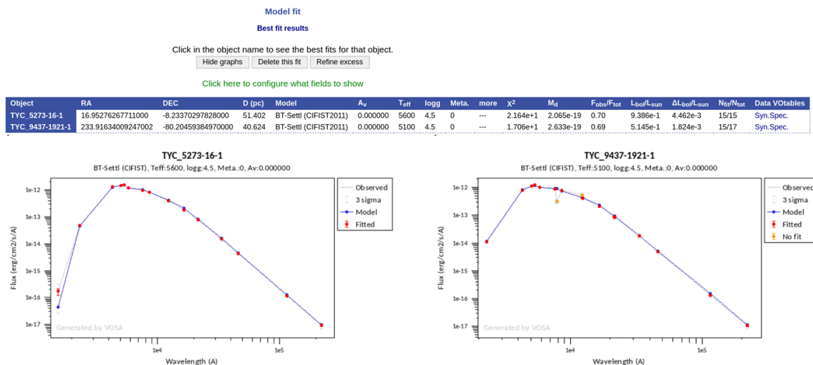
Figure 4. VOSA SED fitting
