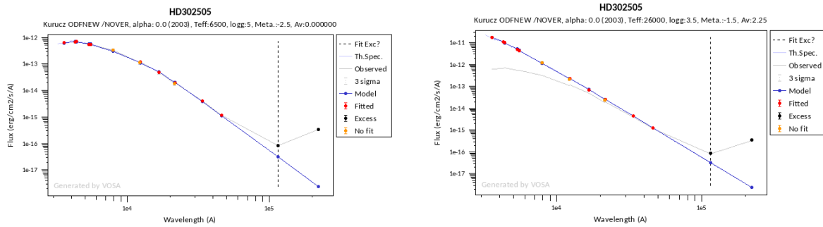
Figure 10. Plot of the SED fitting before and after correcting from interstellar extinction ( Step 12 ).
