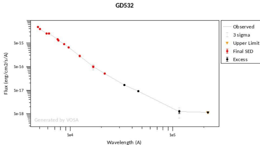
Figure 7. Plot of the photometric data, obtained in Step 5, showing the photometric points affected by infrared excess (black dots).
