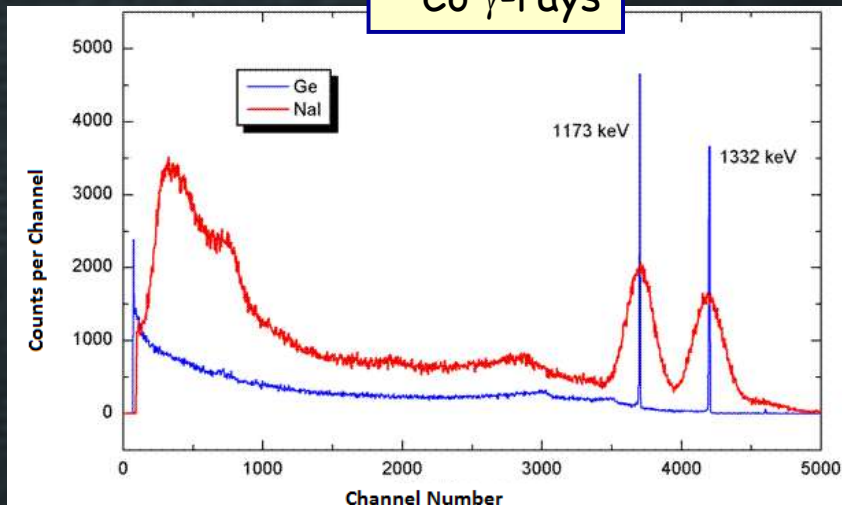
^{60}\text{Co} \gamma -rays
