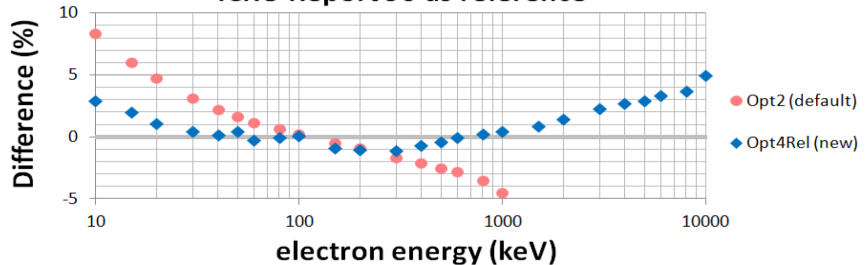
ICRU Report 90 as reference
