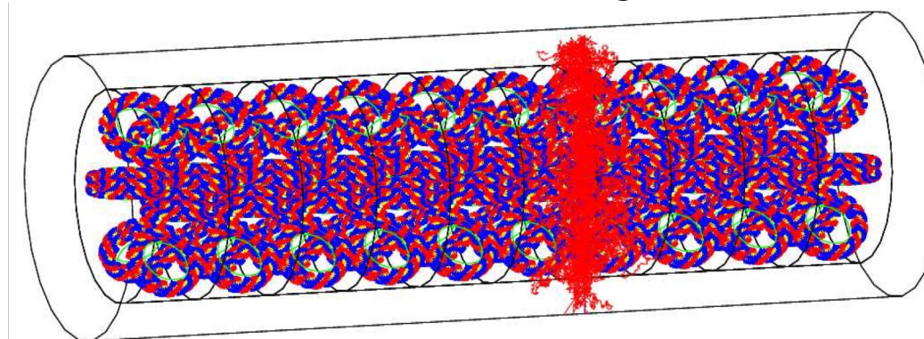
DNA and tracks of 500 keV He^+
