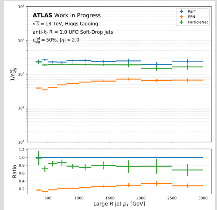
Fig. 24: QCD rejection vs signal efficiency and for all p_T spectra at 50% sig eff for Higgs jets .
