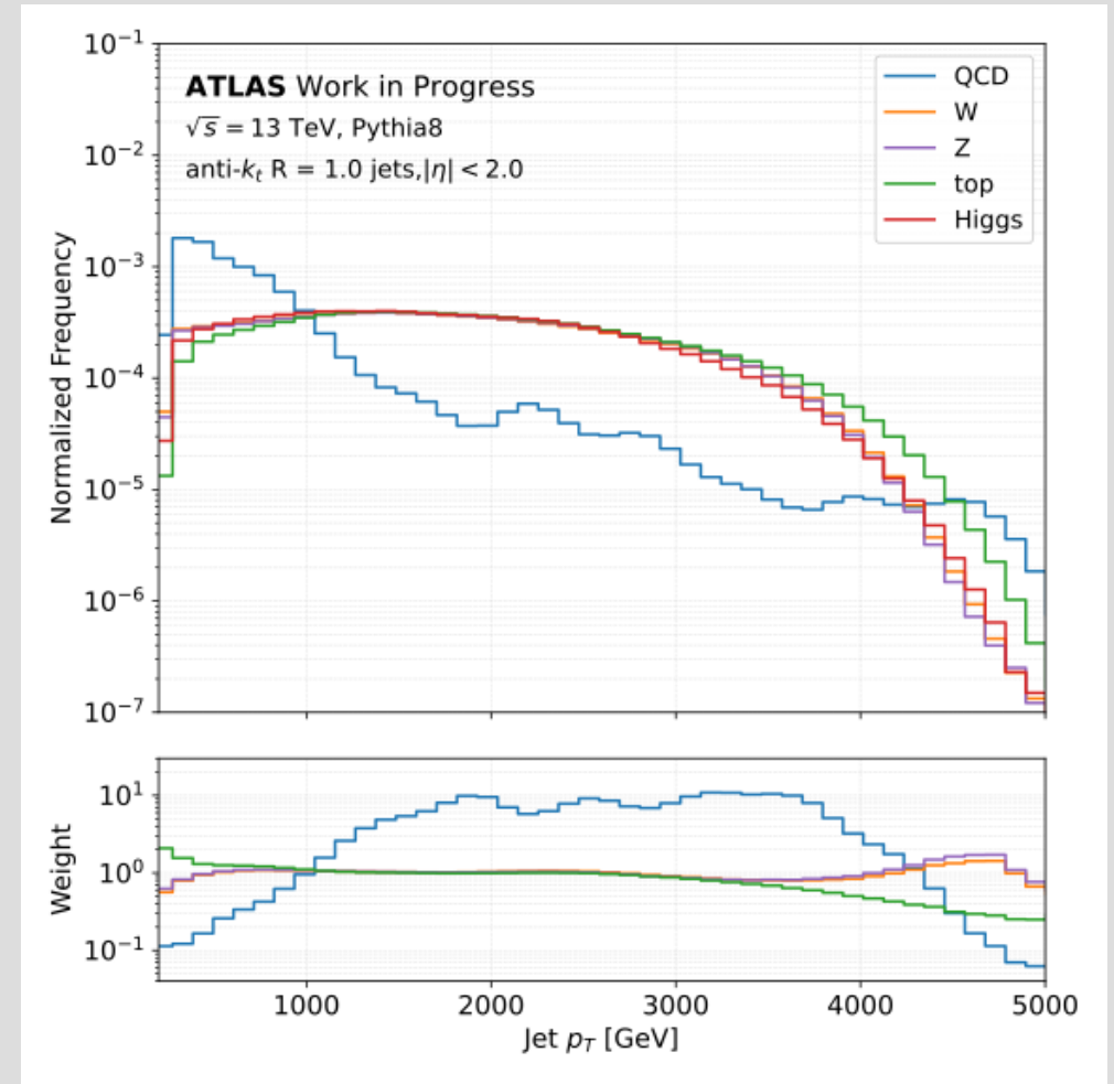
Fig. 17: p_T distribution per jet and weights applied during training.
