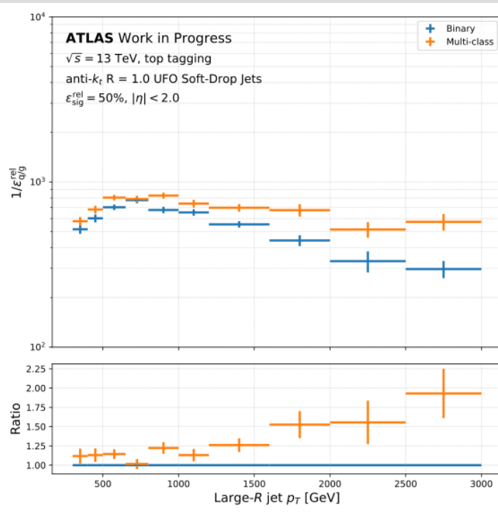
Fig. 30: QCD rejection vs signal efficiency and for all p_T spectra at 50% sig eff for top jets .
