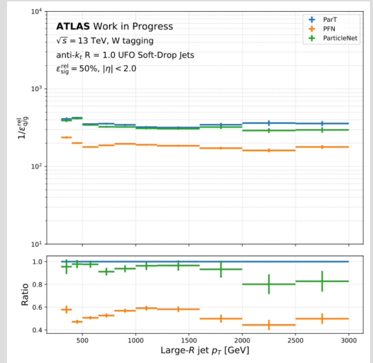
Fig. 22: QCD rejection vs signal efficiency and for all p_T spectra at 50% sig eff for W jets.
