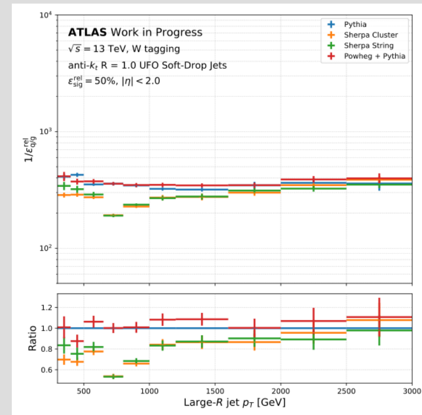
Fig. 11: QCD rejection vs signal efficiency and for all p_T spectra at 50% sig eff for W jets.
