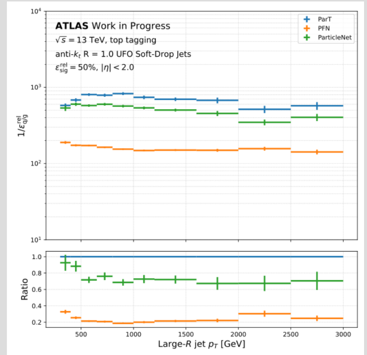
Fig. 23: QCD rejection vs signal efficiency and for all p_T spectra at 50% sig eff for top jets .
