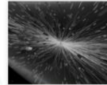
Particle physics
