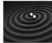
Gravitational waves
