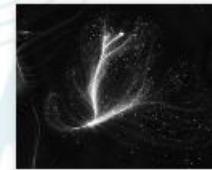
Cosmology
