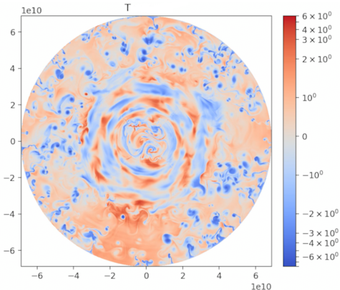
Figure 1: Convection solaire 2d
