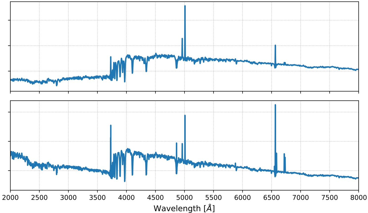
Emission Line (Blue) Galaxy
