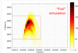
Longitudinal phase space @ 2.86 GeV
