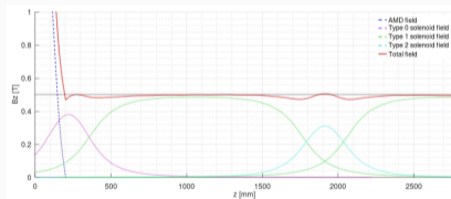
On-axis B_z of different components
