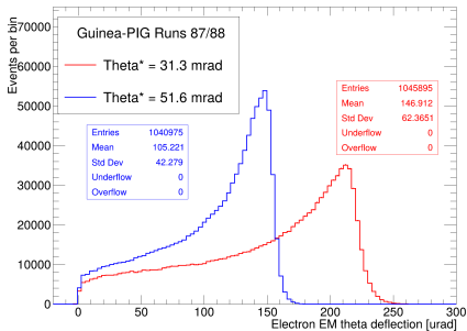
ILCZ Beam Parameters (GP Simulation)
