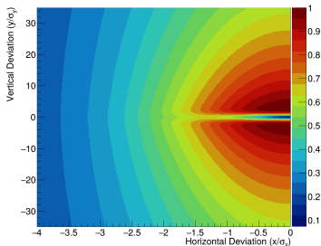
LEP Electric Field Strength
