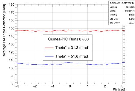
ILCZ Beam Parameters (GP Simulation)
