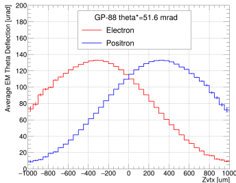
ILCZ Beam Parameters (GP Simulation)
