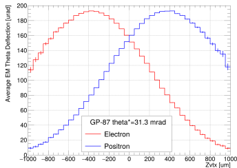
ILCZ Beam Parameters (GP Simulation)
