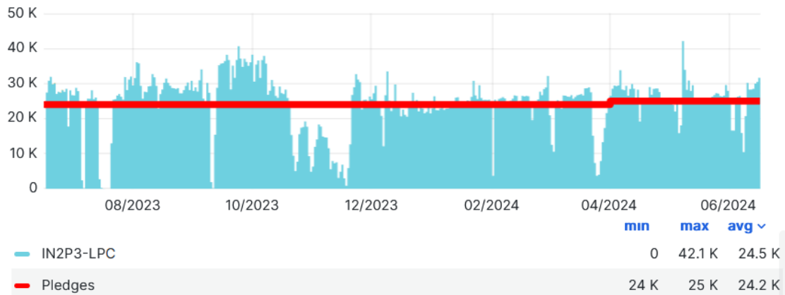
Slots of Running jobs (HS23) ⓘ
