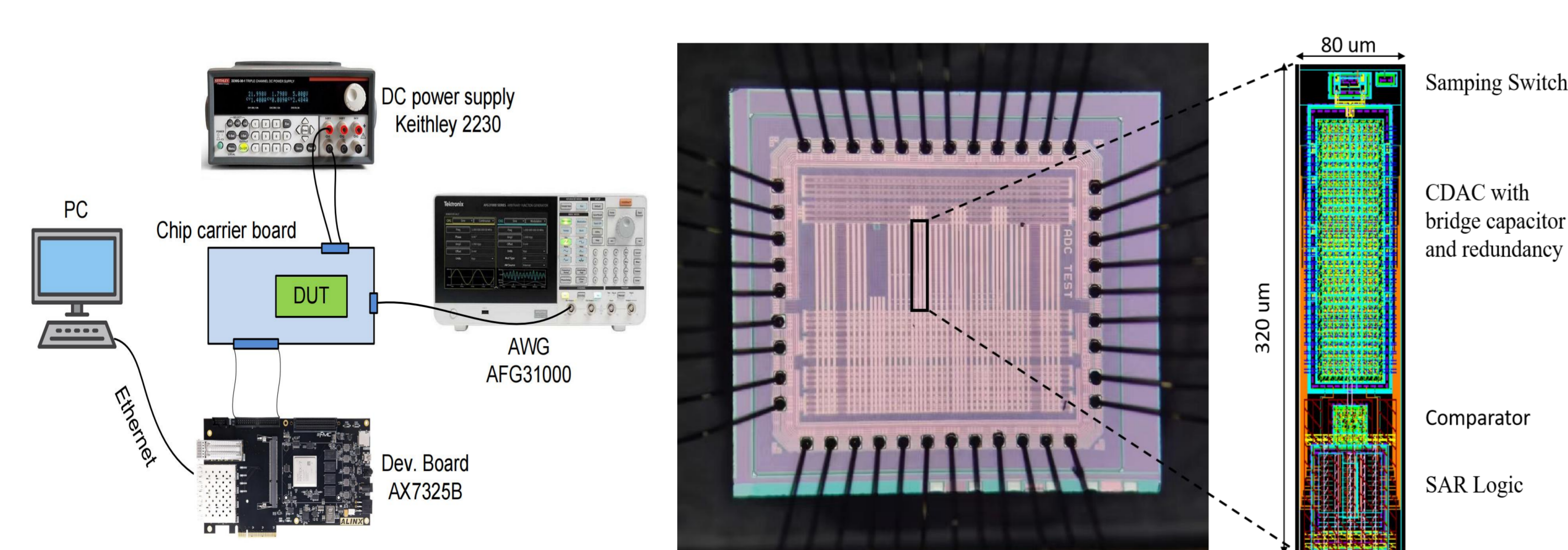
Figure 3. The measurement setup.
