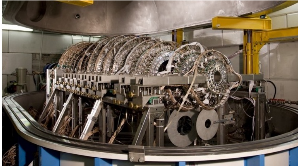
CHIMERA (Charged Heavy-Ion Mass and Energy Resolving Array)
