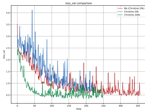
Validation
