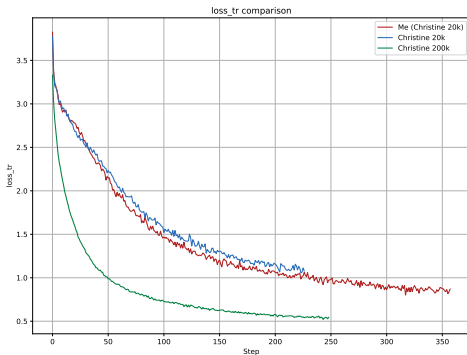
Training
