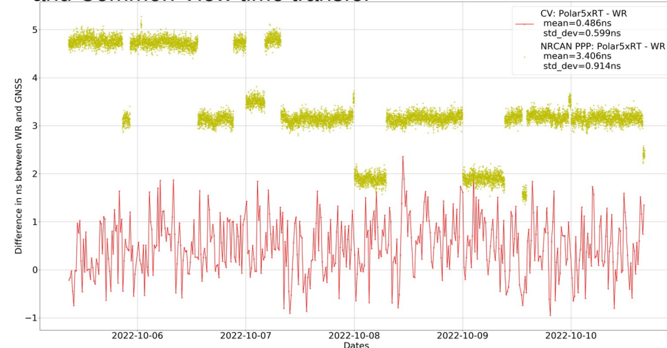
Difference (in ns) between White Rabbit signal from SYRTE and Common View time transfer
