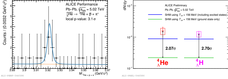
Figure 2. Left panel: Invariant mass distribution of the {}^4_{\Lambda}\overline{\text{He}} in 0–10% most central Pb–Pb collisions at \sqrt{s_{\text{NN}}} = 5.02 TeV. The data points are fitted with a function which is a combination of KDE signal and an exponential background. Right panel: Integrated yields of {}^4_{\Lambda}\text{He} and {}^4_{\Lambda}\text{H} in 0–10% most central Pb–Pb collisions at \sqrt{s_{\text{NN}}} = 5.02 TeV with SHM predictions.
