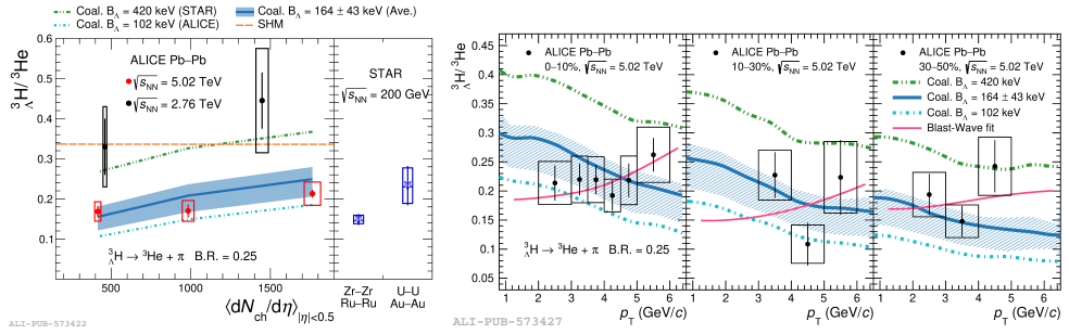
Figure 1. Yield ratio of {}^3_\Lambda\text{H} to {}^3\text{He} in Pb–Pb collisions together with theoretical predictions. Left panel: {}^3_\Lambda\text{H}/{}^3\text{He} as a function of charged-particle multiplicity density \langle dN_{ch}/d\eta \rangle . The recent experimental results of STAR are shown alongside for comparison. Right panel: {}^3_\Lambda\text{H}/{}^3\text{He} versus p_T in different centrality intervals.
