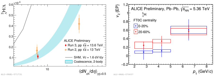
Figure 3. Left panel: Yield ratio of {}^3_{\Lambda}\text{H} to \Lambda in pp collisions with theoretical predictions. The results of {}^3_{\Lambda}\text{H} are obtained from antimatter only. Right panel: v_2 of {}^3_{\Lambda}\text{H} in Pb–Pb collision at \sqrt{s_{\text{NN}}} = 5.36 TeV in different centrality classes.
