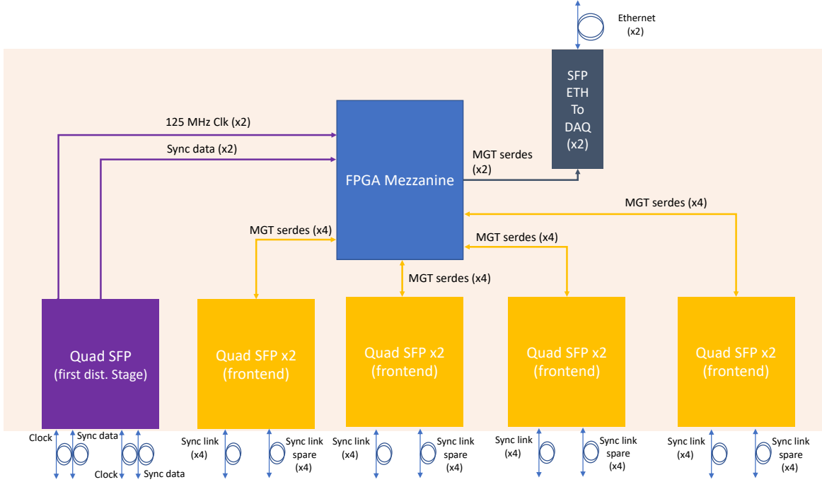
Figure 14: A block scheme of the second distribution stage. The module's is controlled by an FPGA mezzanine (blue box) which has links with other time distribution's entities via optical fibers (blue lines with circles) in turn connected via SFP (small form factor pluggable) electro-optical transceivers to the FPGA high speed serial lines (MGT). Each quad SFP block contains 4 bidirectional fiber connections to front-ends (yellow boxes) and first distribution stage (purple box).
