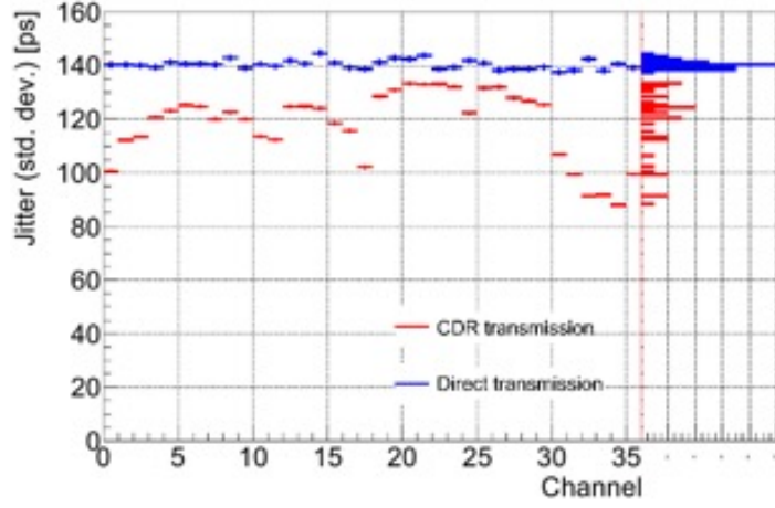
Figure 21: TDC resolution of a QTC receiving the clock from a clock and data recovery scheme (CDR, red dots) compared with the setup in which the clock is feed directly on a dedicated fiber (direct, blue dots) .
