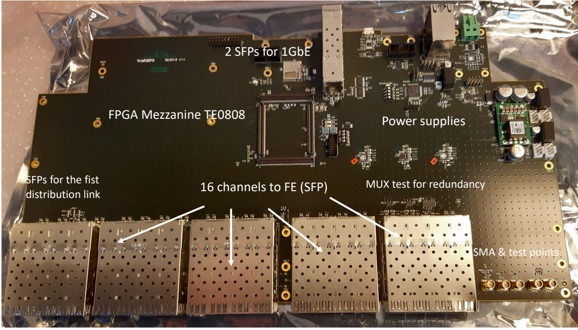
Figure 22: First stage time distribution module prototype board layout.
