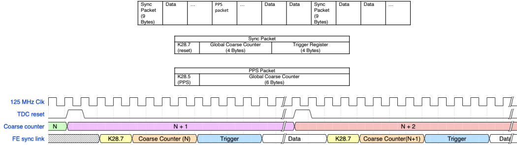
Figure 23: The sync and PPS packets. The top part contains an example of the data stream where a sync packet and a PPS packet are sent along with the non-synchronous data and the detail of the two packets. The time diagram of the bottom part highlights the time relation between the TDC reset and the synchronous packet.
