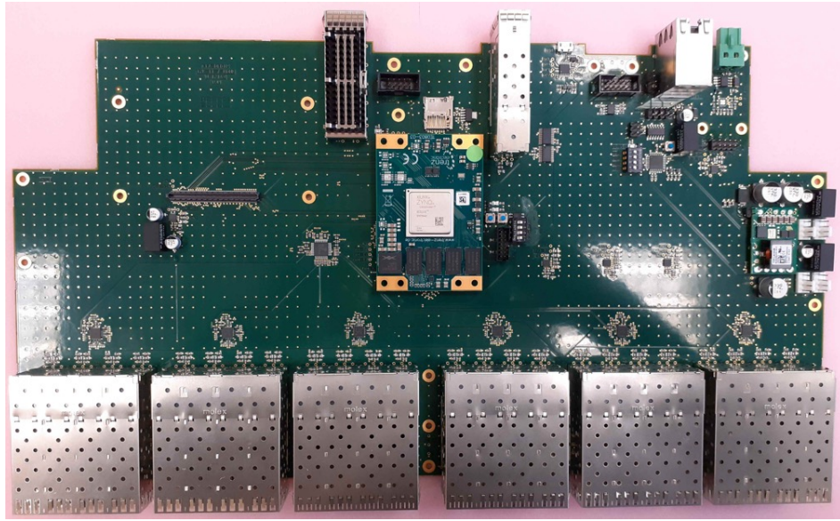
Figure 13: Picture of the RDHK motherboard and the installed SoM.
