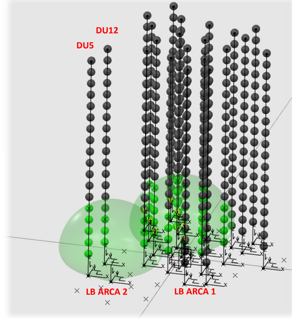
Already Deployed DUs – 3D view to scale (except DOMs)
