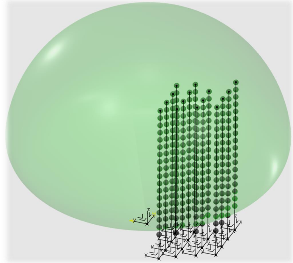
Already Deployed DUs – 3D view to scale (except DOMs)
