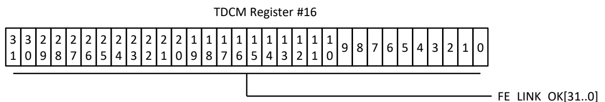
Fig. 60. Front-End Link OK Register #16.
