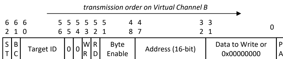
Fig. 36. TDCM to FE Virtual Channel B frame format.
