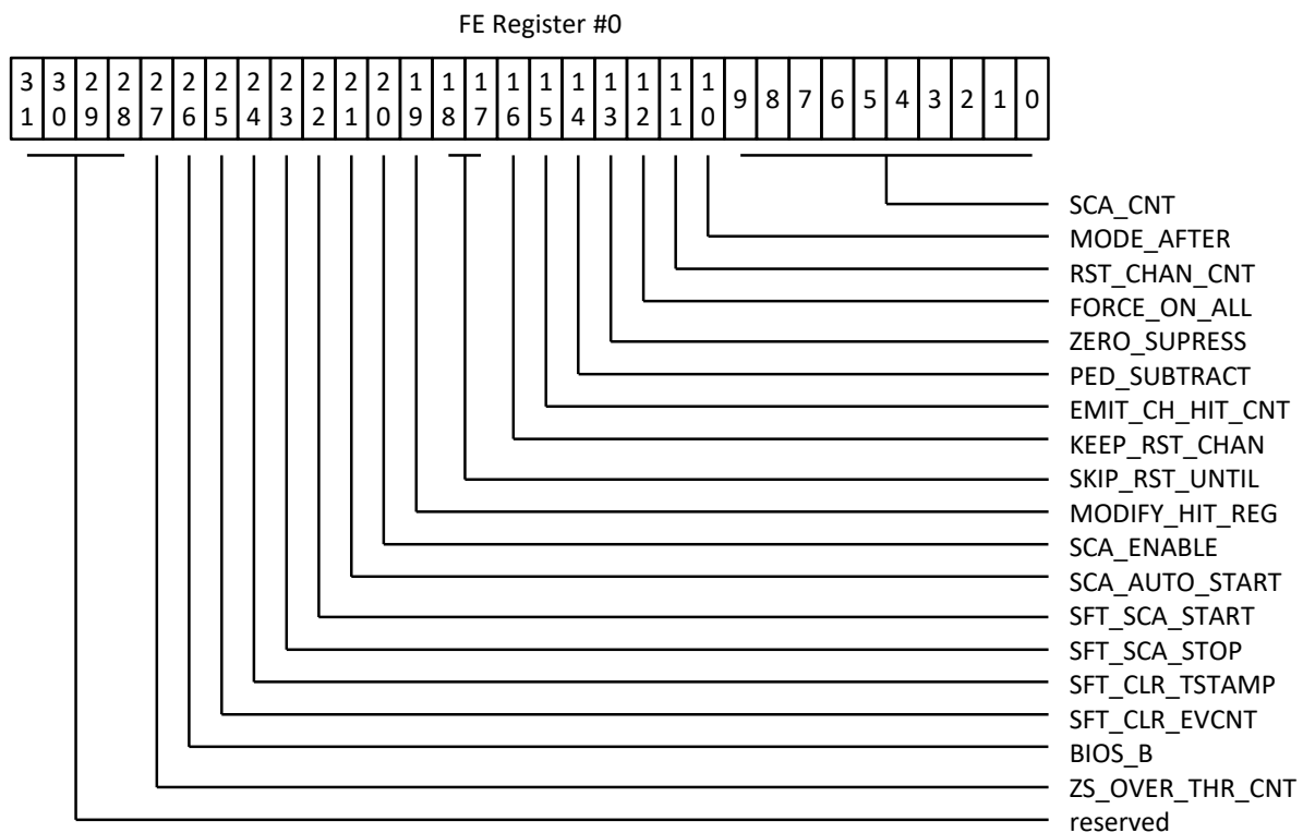
Fig. 80. General Configuration Register (Register#0).
