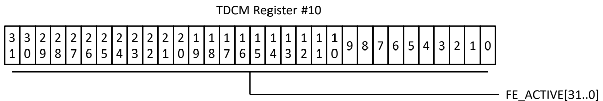
Fig. 56. Front-End active Register #10.
