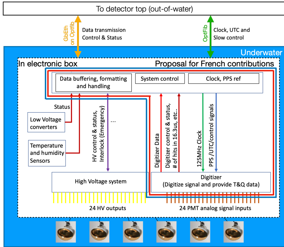
Figure 16: A front end electronics scheme with the functional blocks reported. The intended French contributions are surrounded with a tricolor box.
