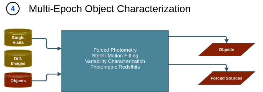
FIGURE 4: Illustration of the conceptual algorithm design for Image Coaddition, Coadded Image Analysis, and Multi-epoch Object Characterization pipelines.
