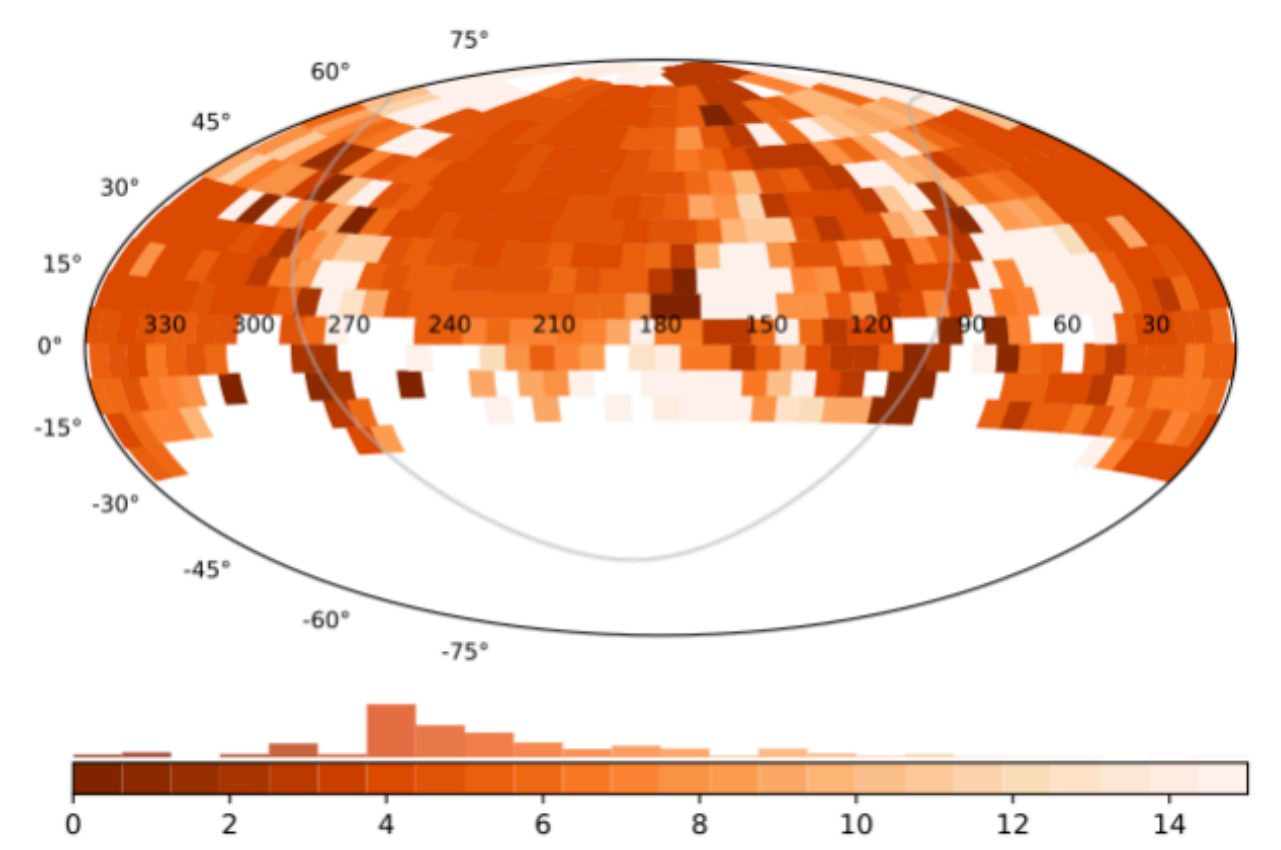
Median delay between two consecutive exposures [days]
