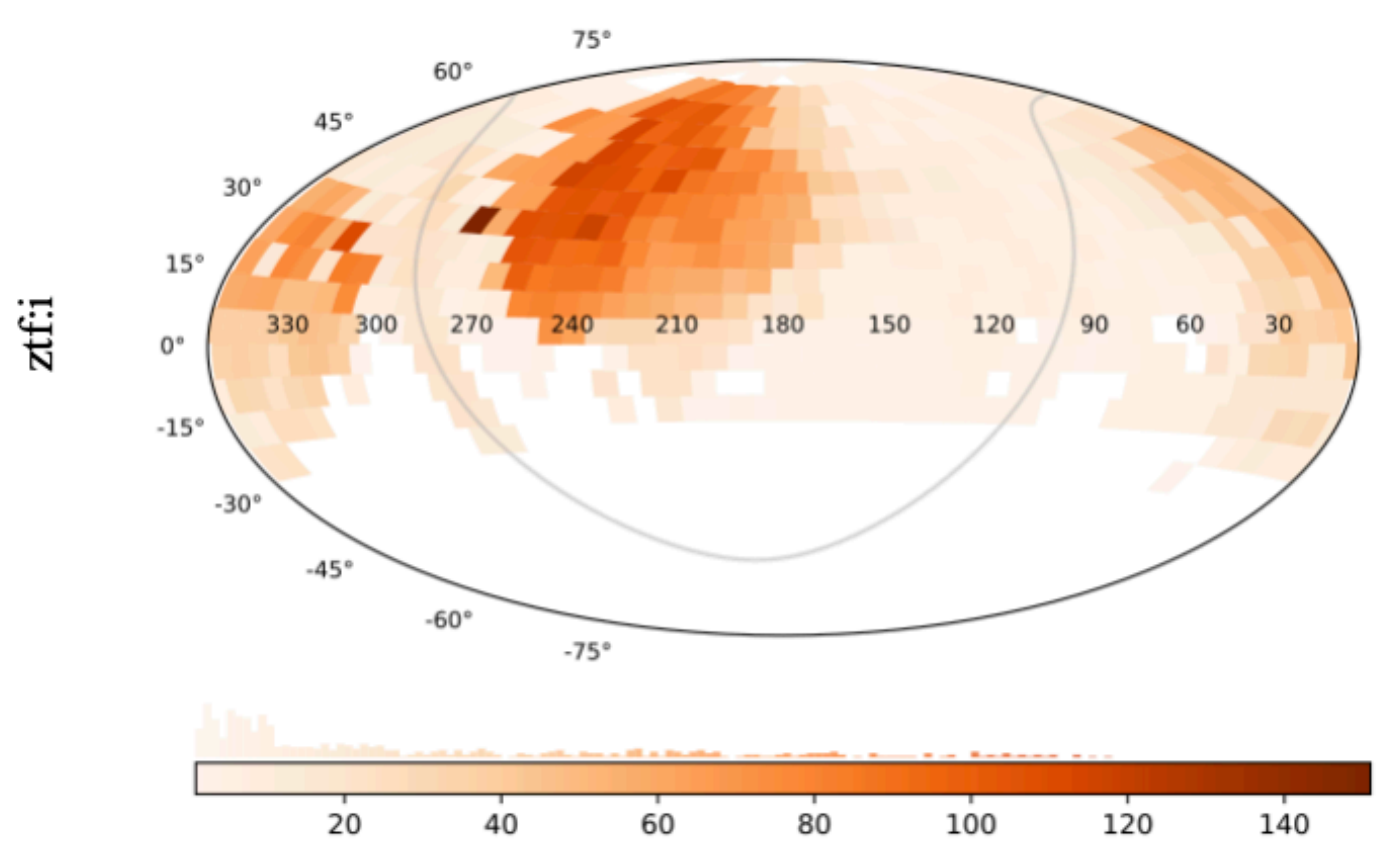
Total number of exposures
