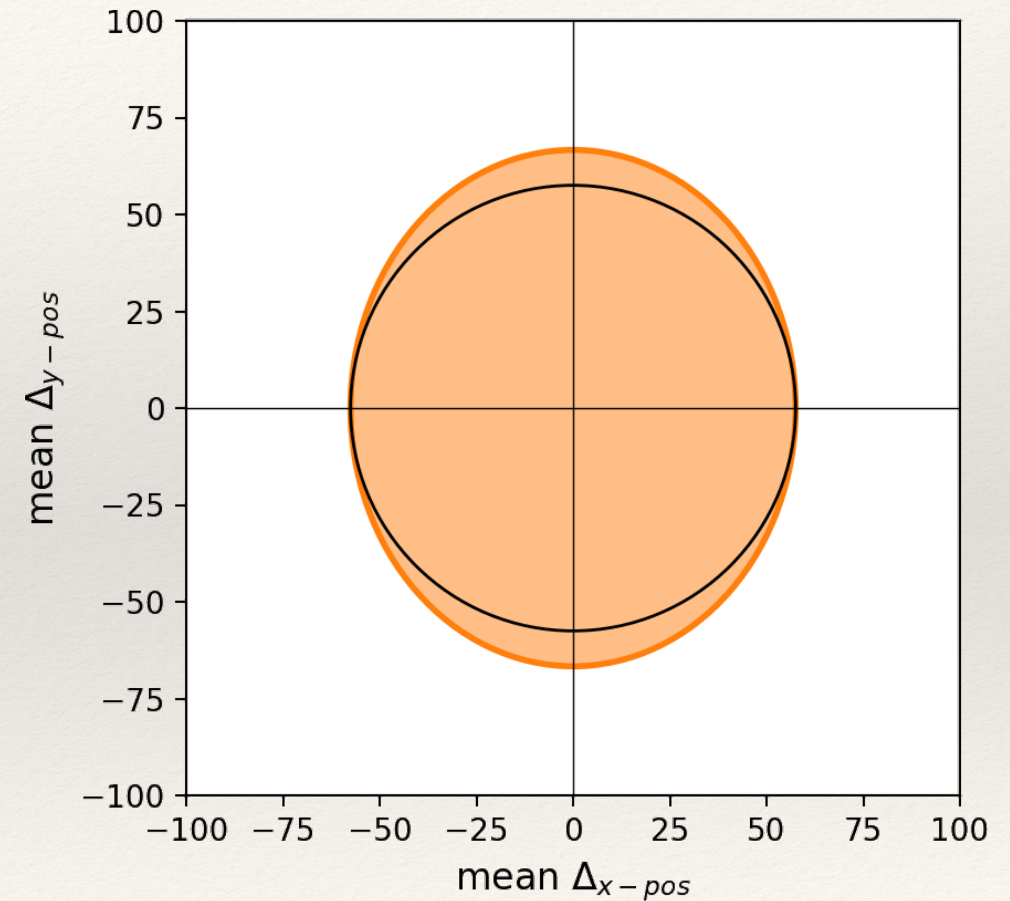
Effective Dithering per field
