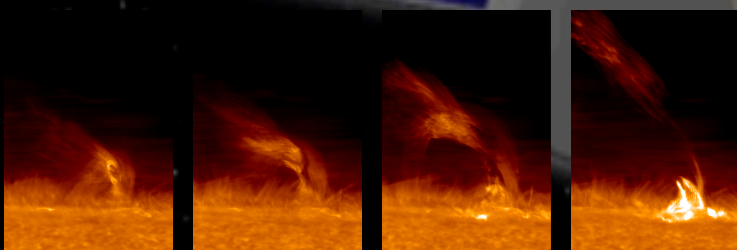
Dynamic plasma ejection in the chromosphere
