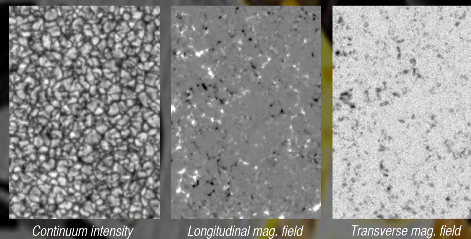
Continuum Intensity Longitudinal mag. field Transverse mag. field
