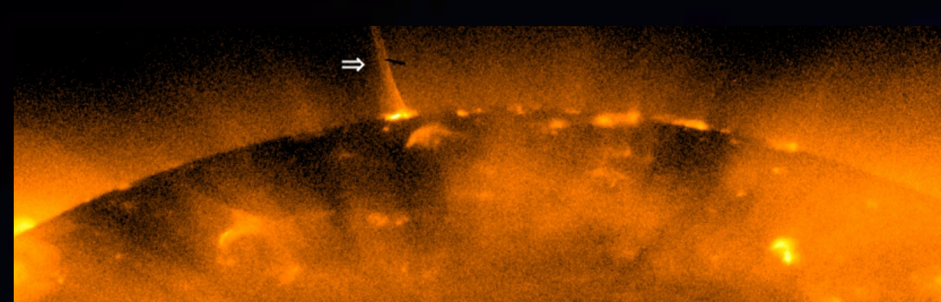
X-ray jet in a polar coronal hole
