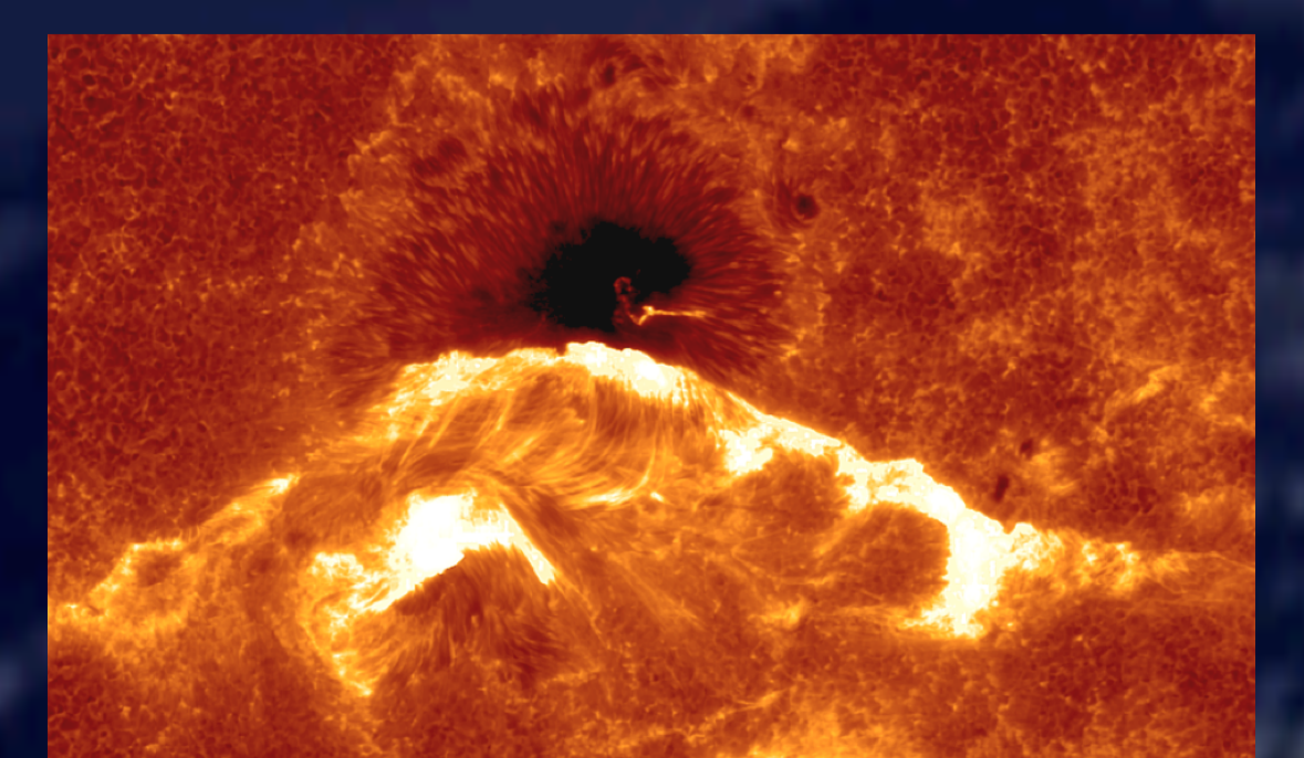
Flare ribbons caused by electron beam bombardment of the chromosphere.
