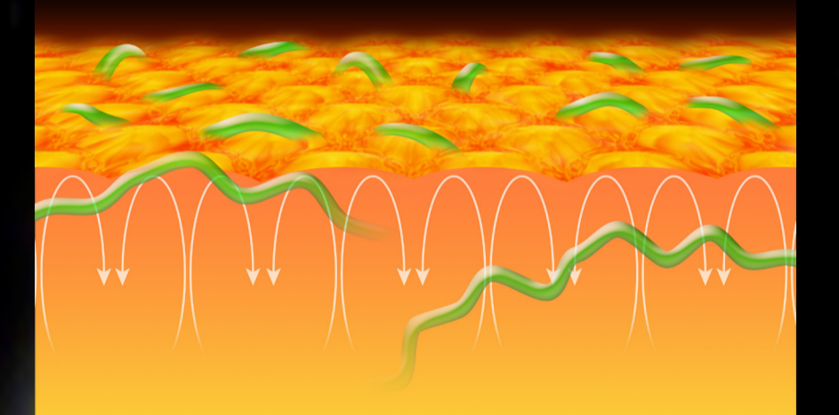
Artist's view of solar convection (granules) and horizontal magnetic fields.
