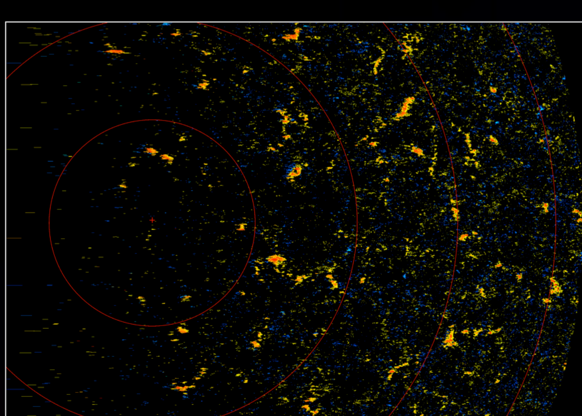
Magnetic landscape of the Sun's pole
