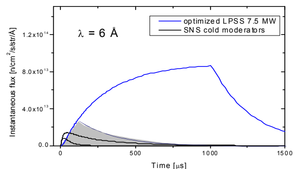
A linac driven long pulse source can emulate with proton pulses of ~ 100 \mu s duration the slow neutron pulses of a short pulses source (grey area vs. black lines), and produce order of magnitude more neutrons per pulse with higher peak brilliance with proton pulse lengths in the ms range.
