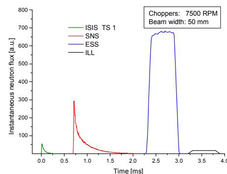
Innovative fast rotating mechanical neutron chopper systems allow us to cut out shorter pulses for better definition of the neutron velocity (energy) from the long ESS pulses. The area of the pulses gives in the figure in this example the performance gain of ESS compared to the existing most powerful neutron sources (J-PARC is about equivalent to SNS).
