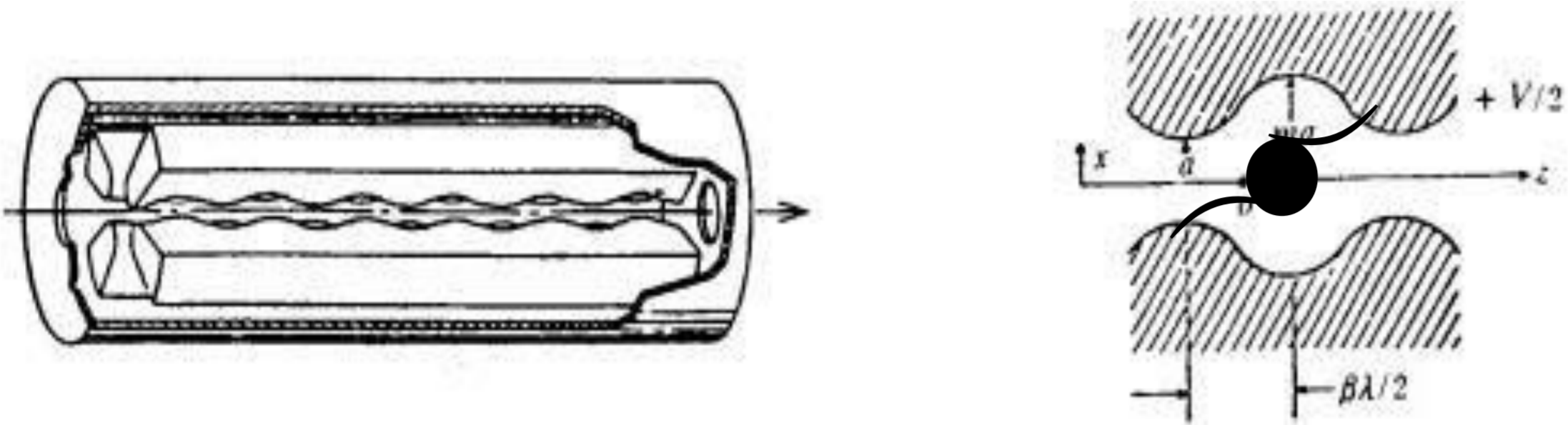
Fig 1: Schematic structure of conventional RFQ
