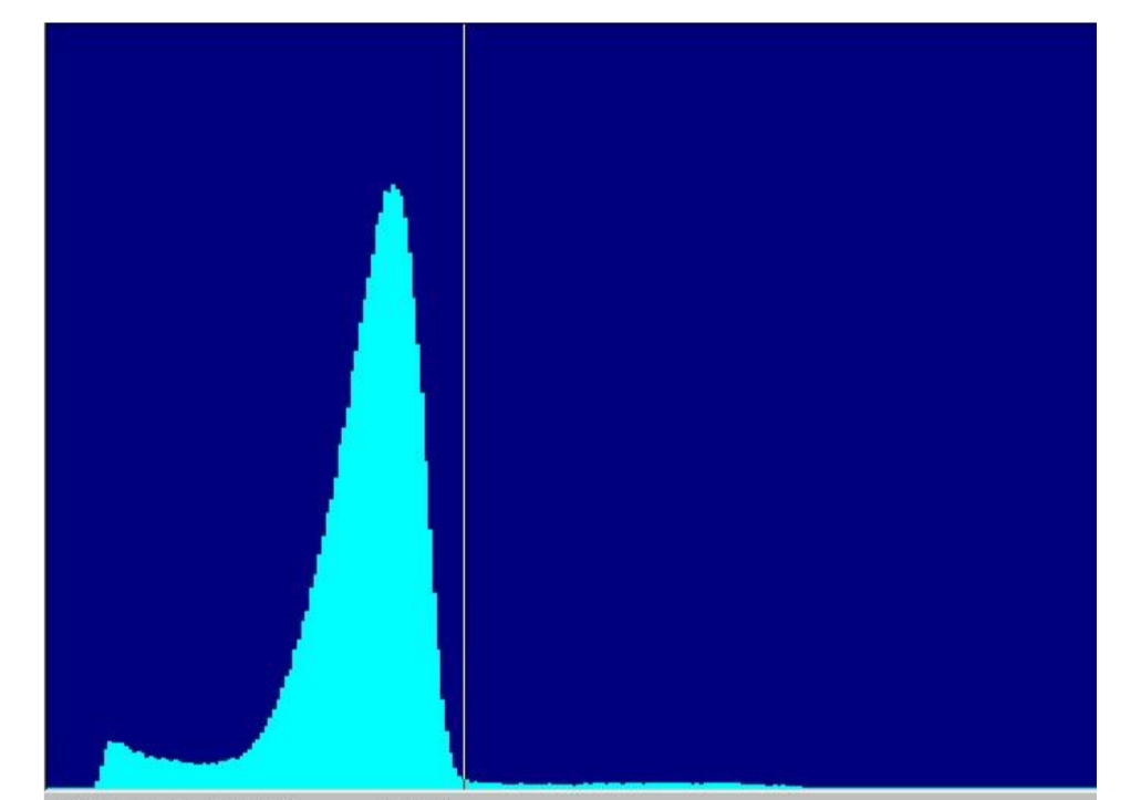
Fig. 7 X-ray spectrum of full power test with 26 MHz RF power source without beam
