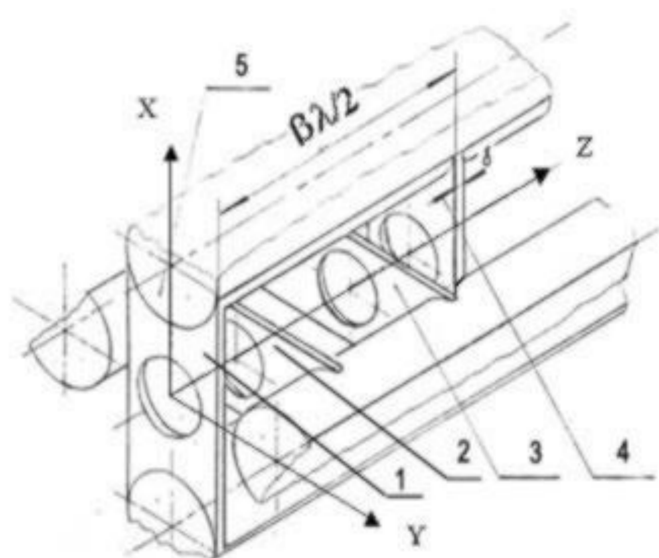
Fig 3: Diaphragms in SFRFQ
