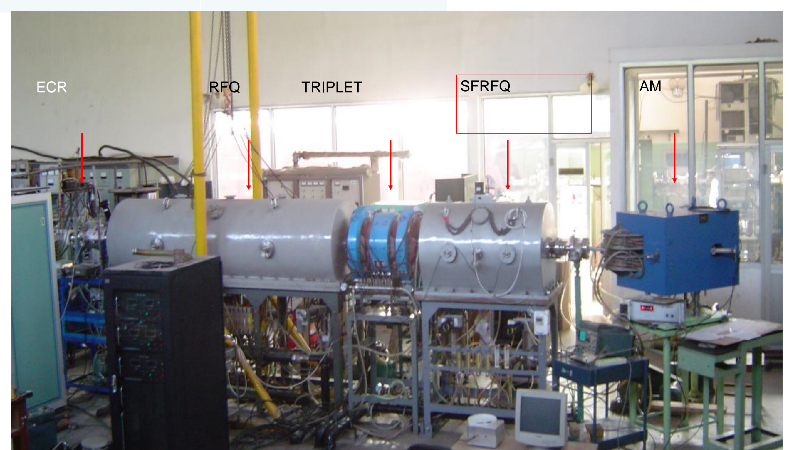
Fig. 8 The Layout of the SFRFQ beam test
