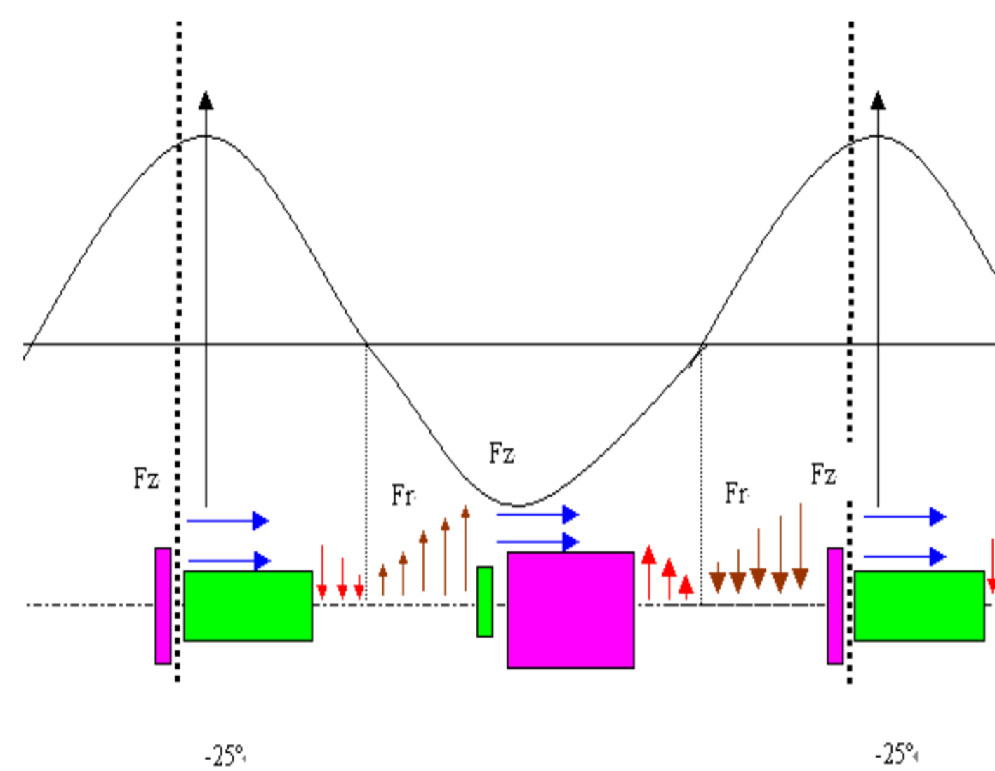
Fig 4: Asymmetry diaphragm system
