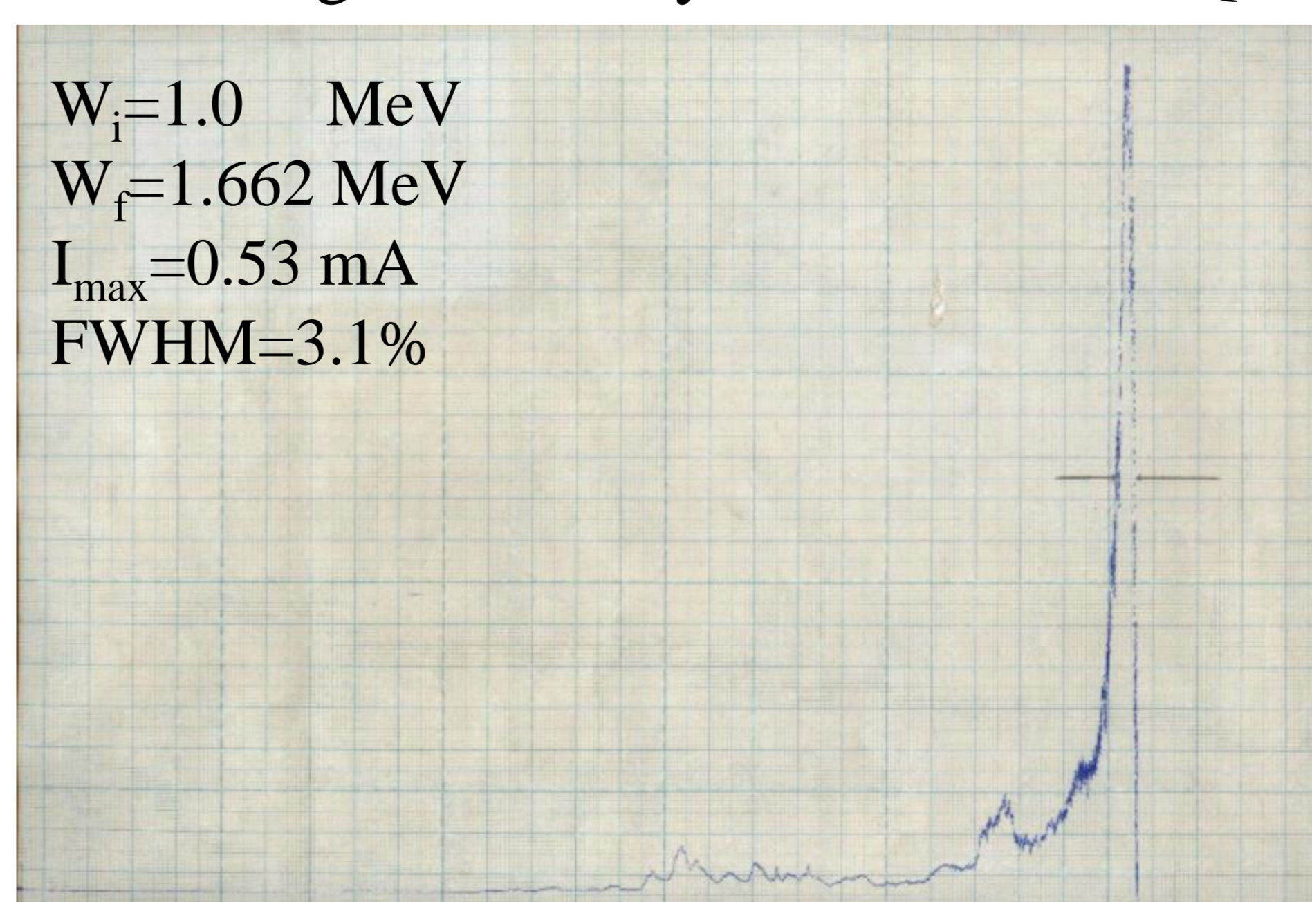
Fig. 9 Output Energy Spectrum of the O^+ beam
