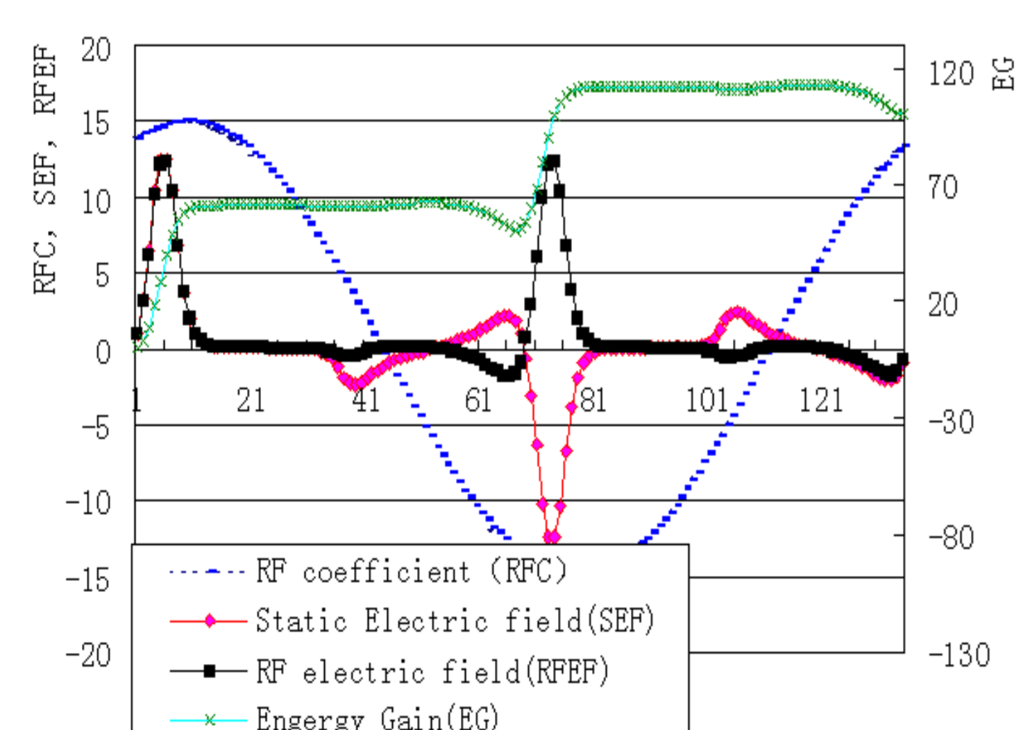
Fig. 5 Energy gain in SFRFQ
