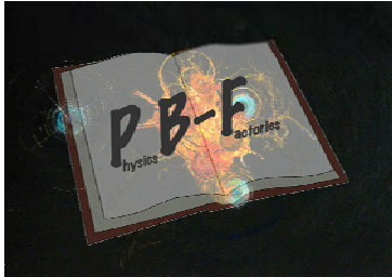
Physics of the B-factories
