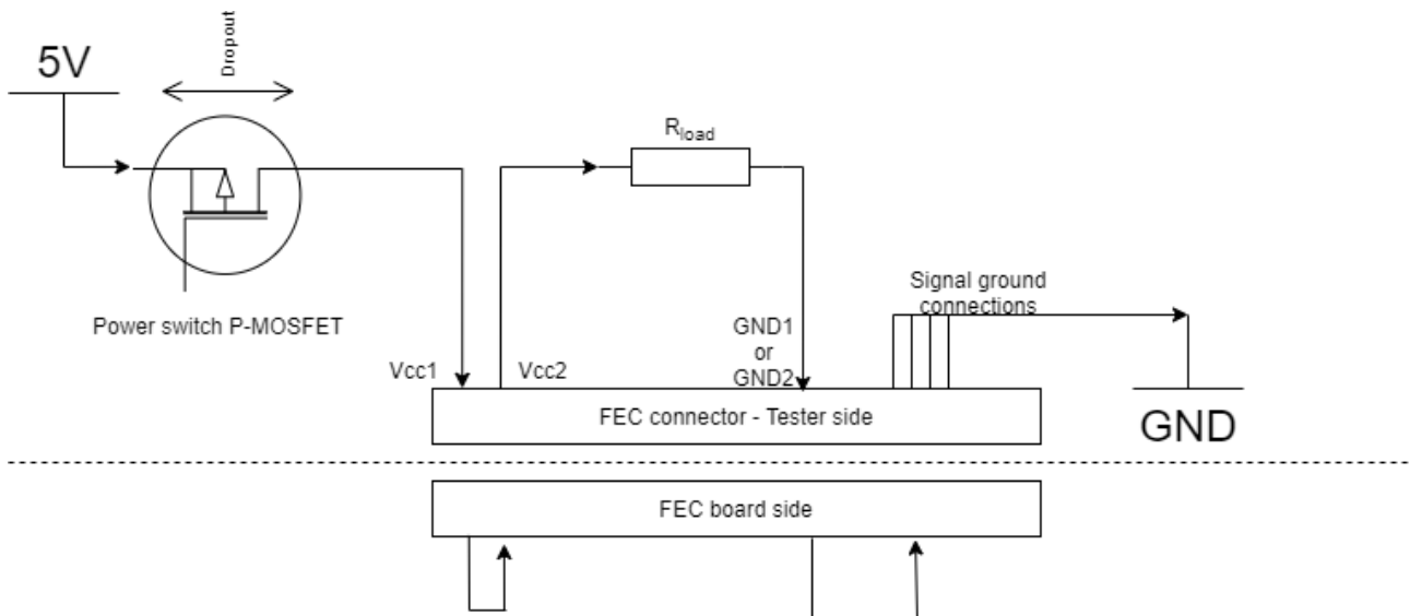
Test current flow on FEC tester board
